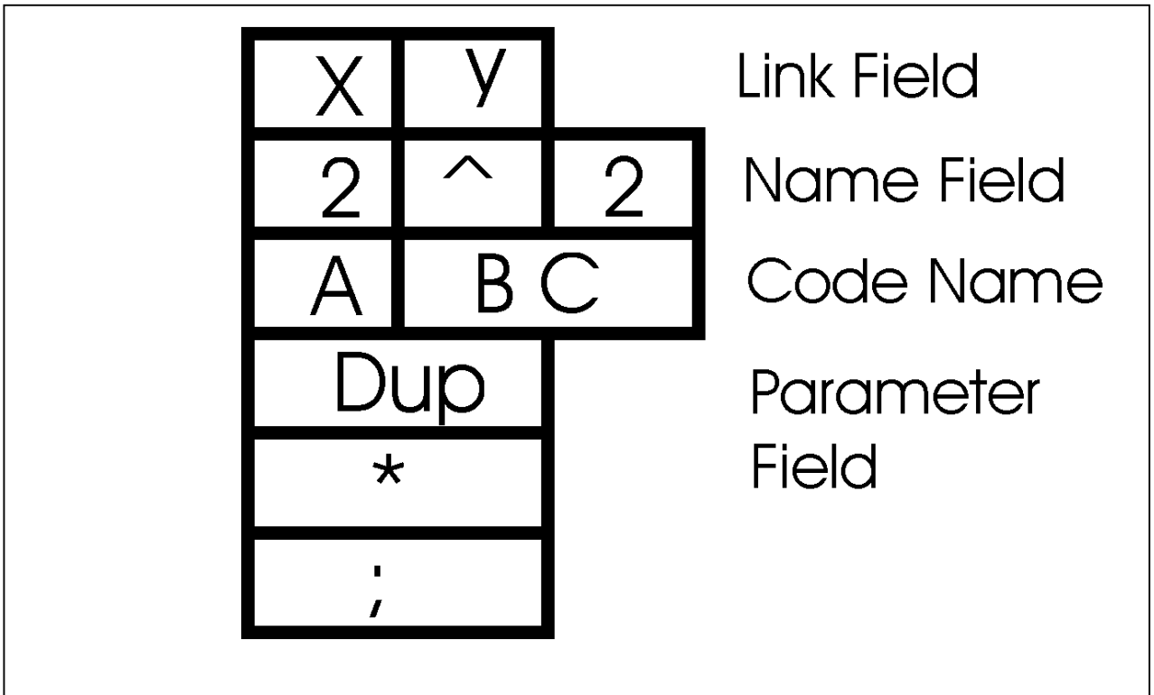
Figure 8: Dictionary entry
