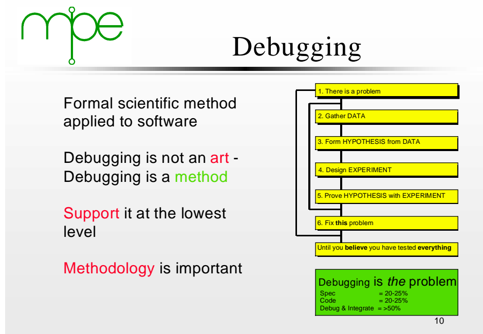
Figure 1: Formal debugging
